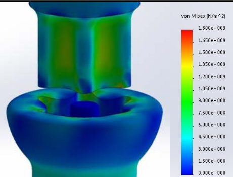
iNTREPID's B-Drive™ Screw Drive System
