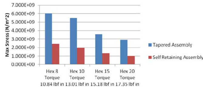
Screw Head Max Stress
