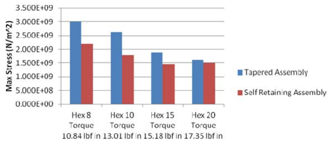
Driver Max Stress
